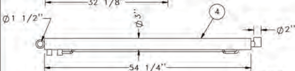
CYLINDRE COLONNE AVANT 48" 48" FRONT POST CYLINDER
